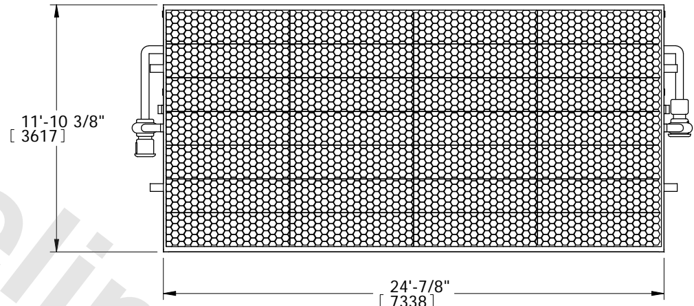
FACE 1 PLAN VIEW
